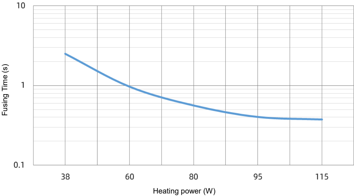
SHP 45 A Power-Time Curve
