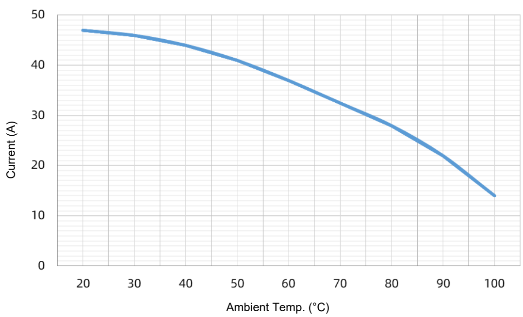
SHP 45 A Current Carrying Capacity
