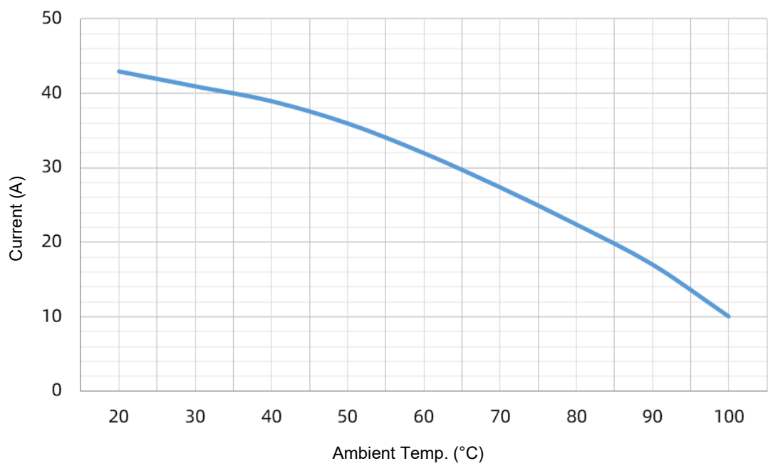
SHP 30 A Current Carrying Capacity
